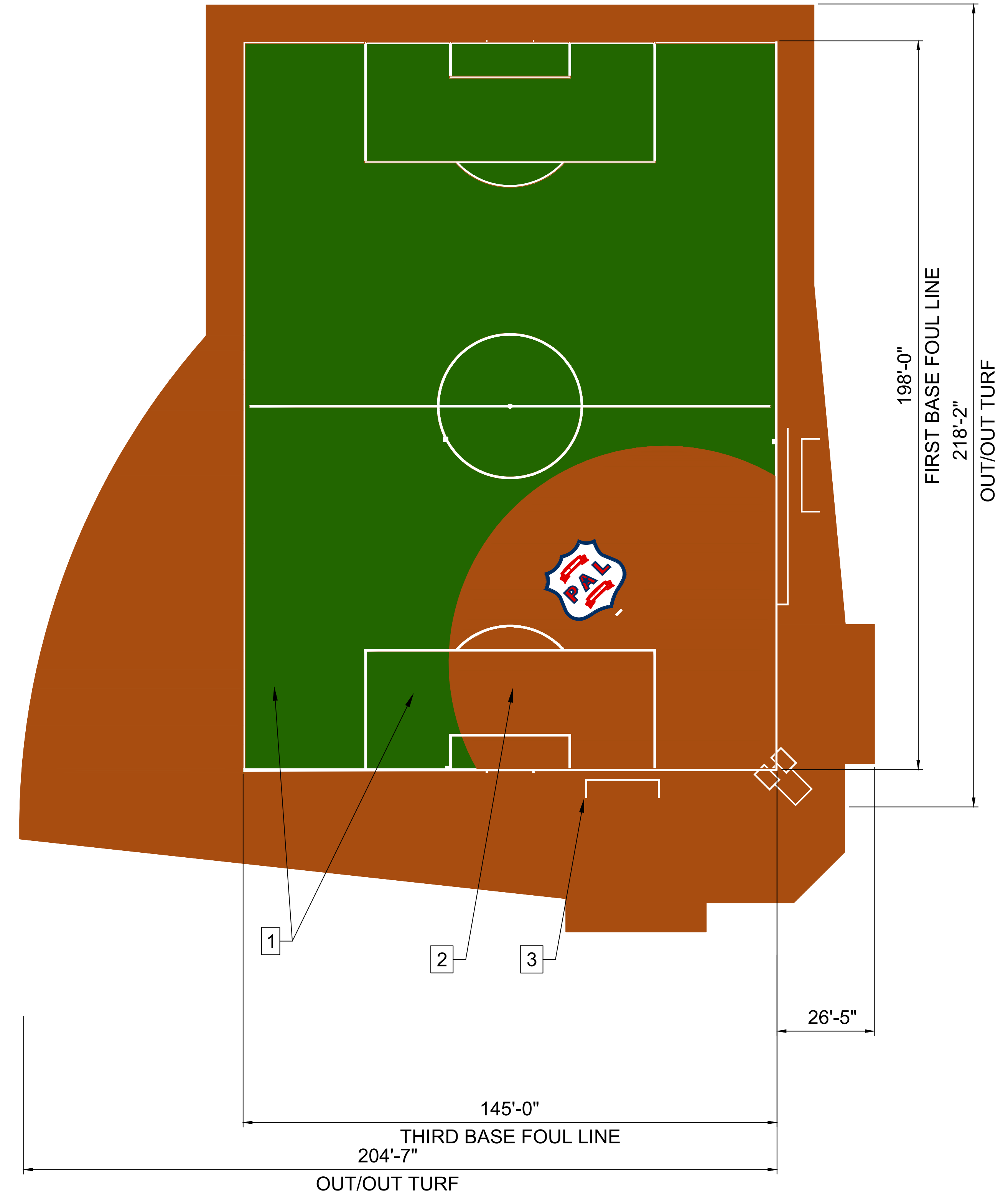
BASEBALL TURF PLAN & COLOR DETAIL
